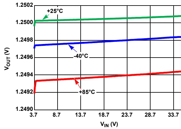
FIGURE 17. DROPOUT WITH -10mA LOAD
