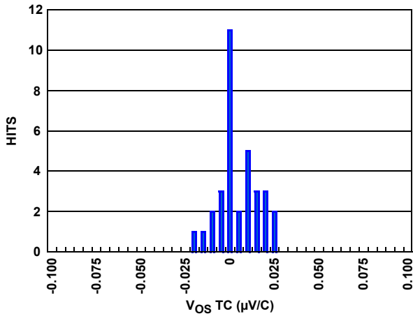
FIGURE 29. AUXILIARY V_{SHUNT} V_{OS} TC (-40°C TO +125°C)
