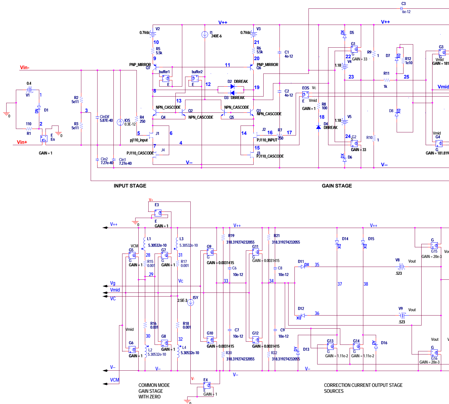
FIGURE 46. SPICE NET LIST
