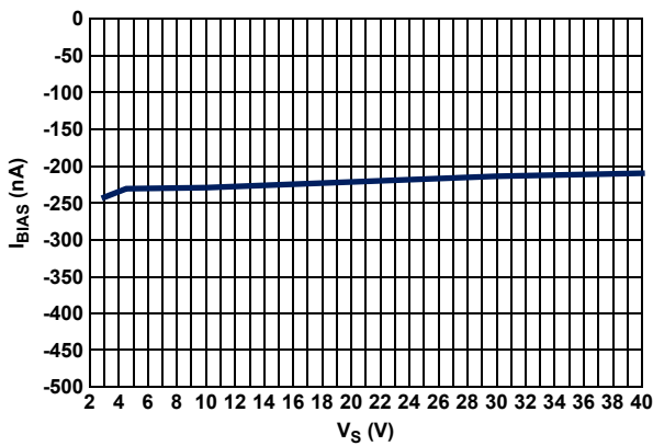
FIGURE 7. I_{BIAS} vs V_S
