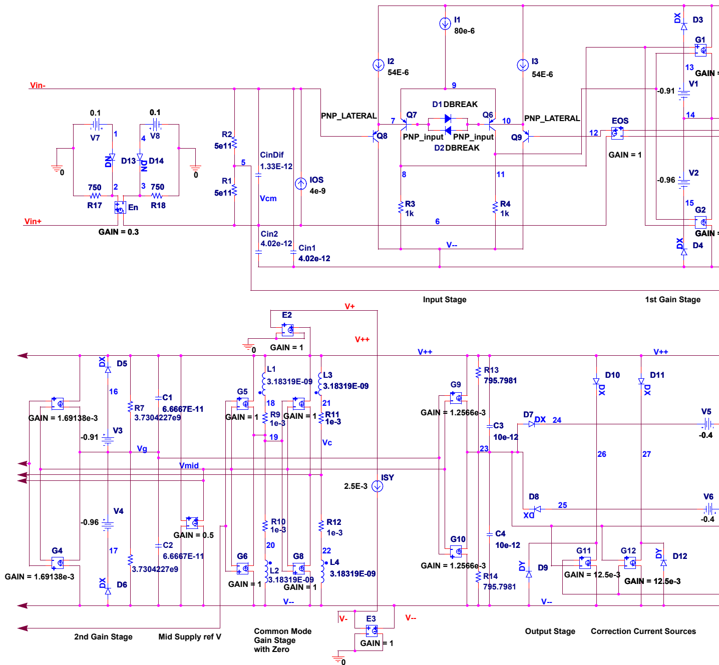
FIGURE 50. SPICE SCHEMATIC
