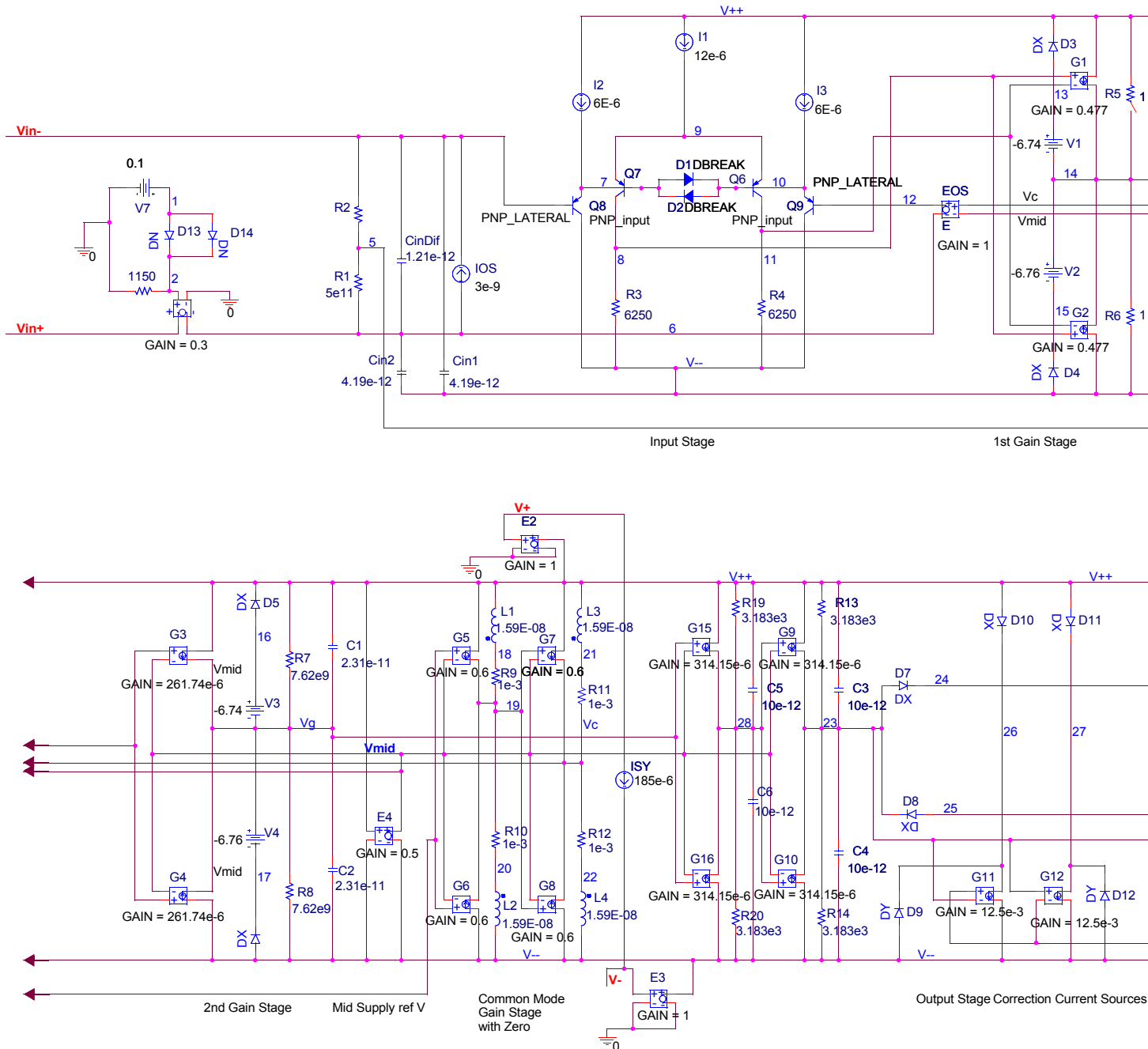
FIGURE 67. SPICE MODEL SCHEMATIC
