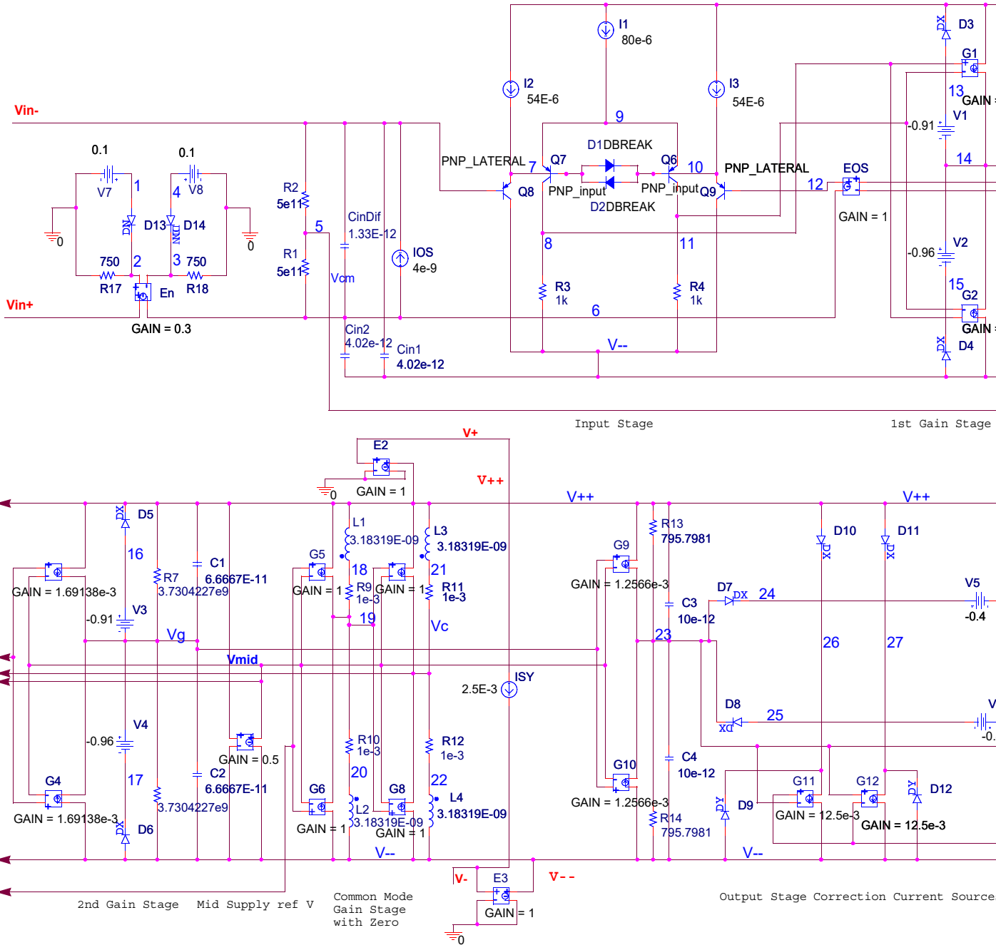
FIGURE 64. SPICE SCHEMATIC
