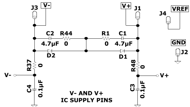
FIGURE 1. POWER SUPPLY CIRCUIT
