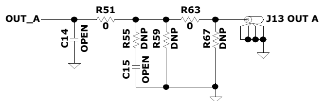
FIGURE 4. OUTPUT STAGE
