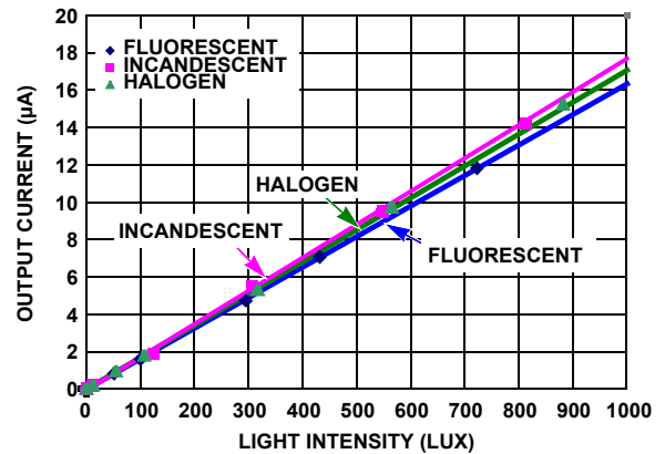
FIGURE 8. OUTPUT CURRENT vs LIGHT INTENSITY
