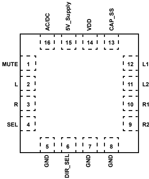
ISL54405 (16 LD \mu TQFN) TOP VIEW
