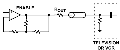
FIGURE 26. DC COUPLE
