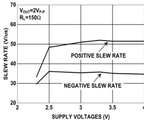
FIGURE 21. SLEW RATE vs SUPPLY VOLTAGE
