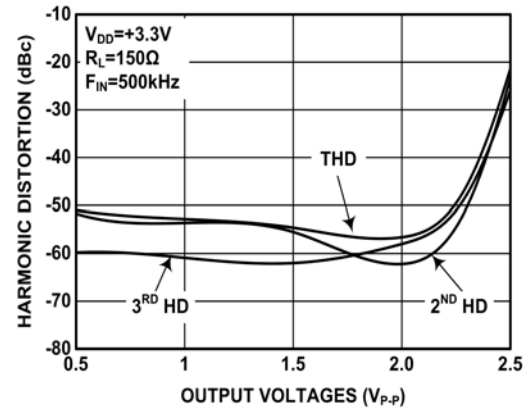
FIGURE 18. HARMONIC DISTORTION vs OUTPUT VOLTAGE
