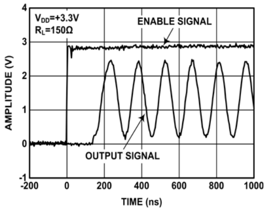
FIGURE 15. ENABLE TIME
