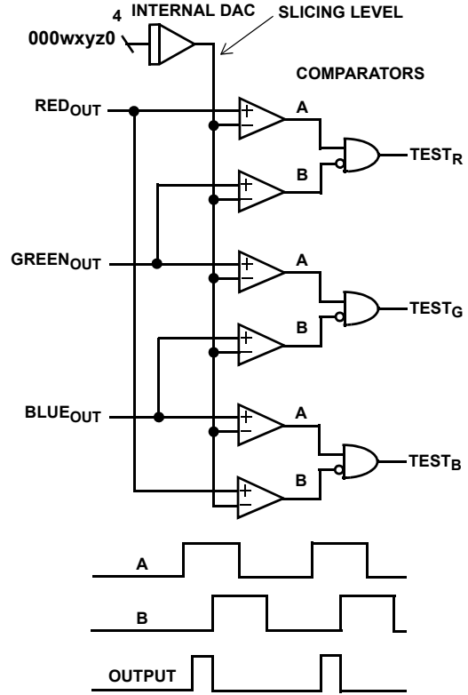
FIGURE 36. DELAY DETECTOR
