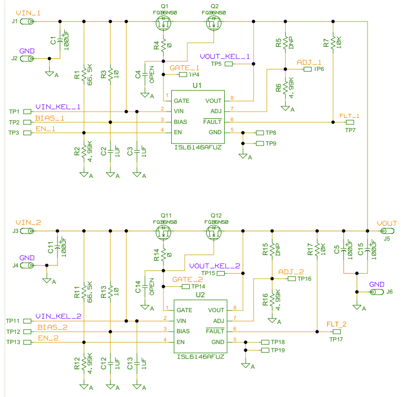
FIGURE 57. ISL6146AEVAL1Z SCHEMATIC
