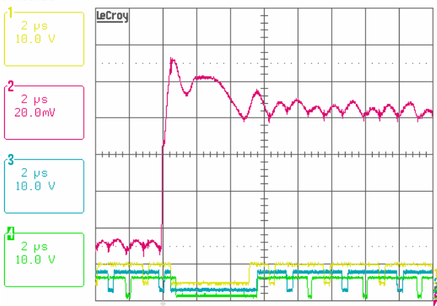
FIGURE 52. LOAD TRANSIENT RESPONSE WITH OVERSHOOT REDUCTION FUNCTION ENABLED, V_{IN} = 12V , SV CLARKSFIELD CPU TEST CONDITION: VID = 0.95V, I_O = 12A/51A , di/dt = "FASTEST", LL = 1.9m \Omega , Ch1: LGATE1, Ch2: V_O , Ch3: LGATE2, Ch4: ISL6208 LGATE
