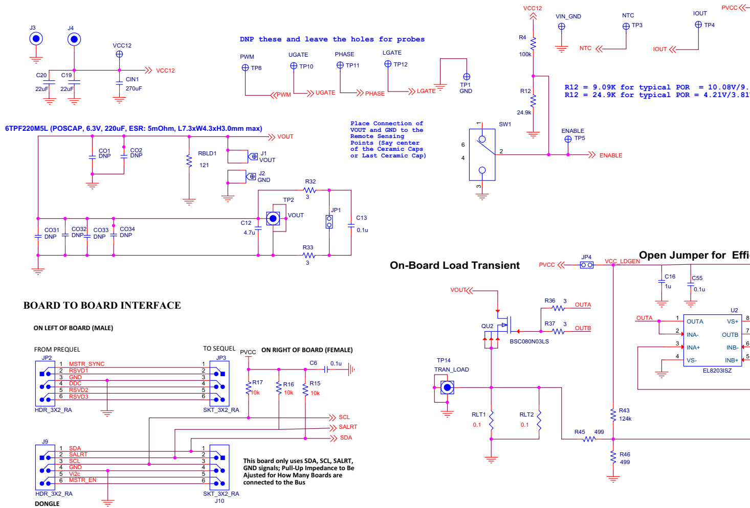
FIGURE 7. I/O CONNECTORS, AUXILIARY CIRCUITS AND ON-BOARD TRANSIENT LOAD SCHEMATICS (2 OF 2)
