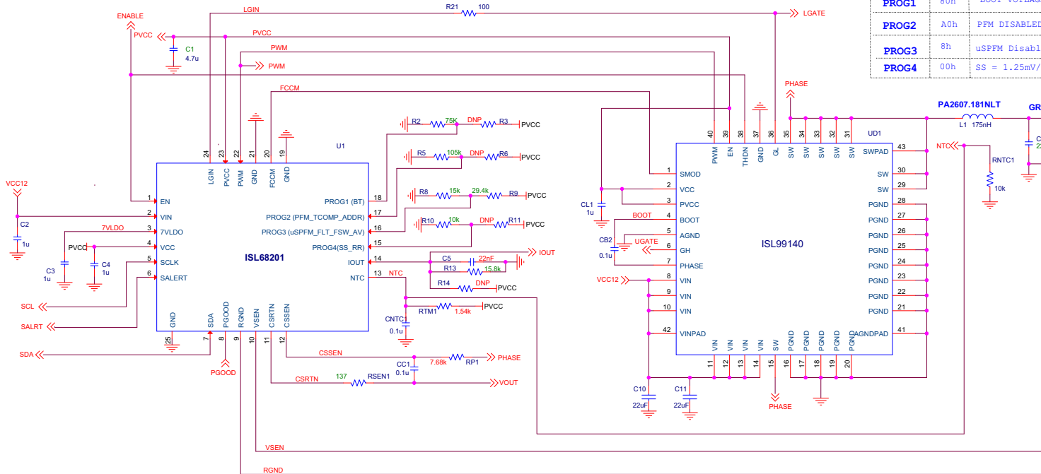
FIGURE 6. ISL68201-99140DEMO1Z 1V AT 35A BUCK SOLUTION SCHEMATICS (1 OF 2)
