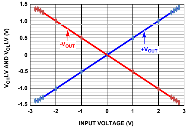
FIGURE 25. V_{OH} AND V_{OL}
