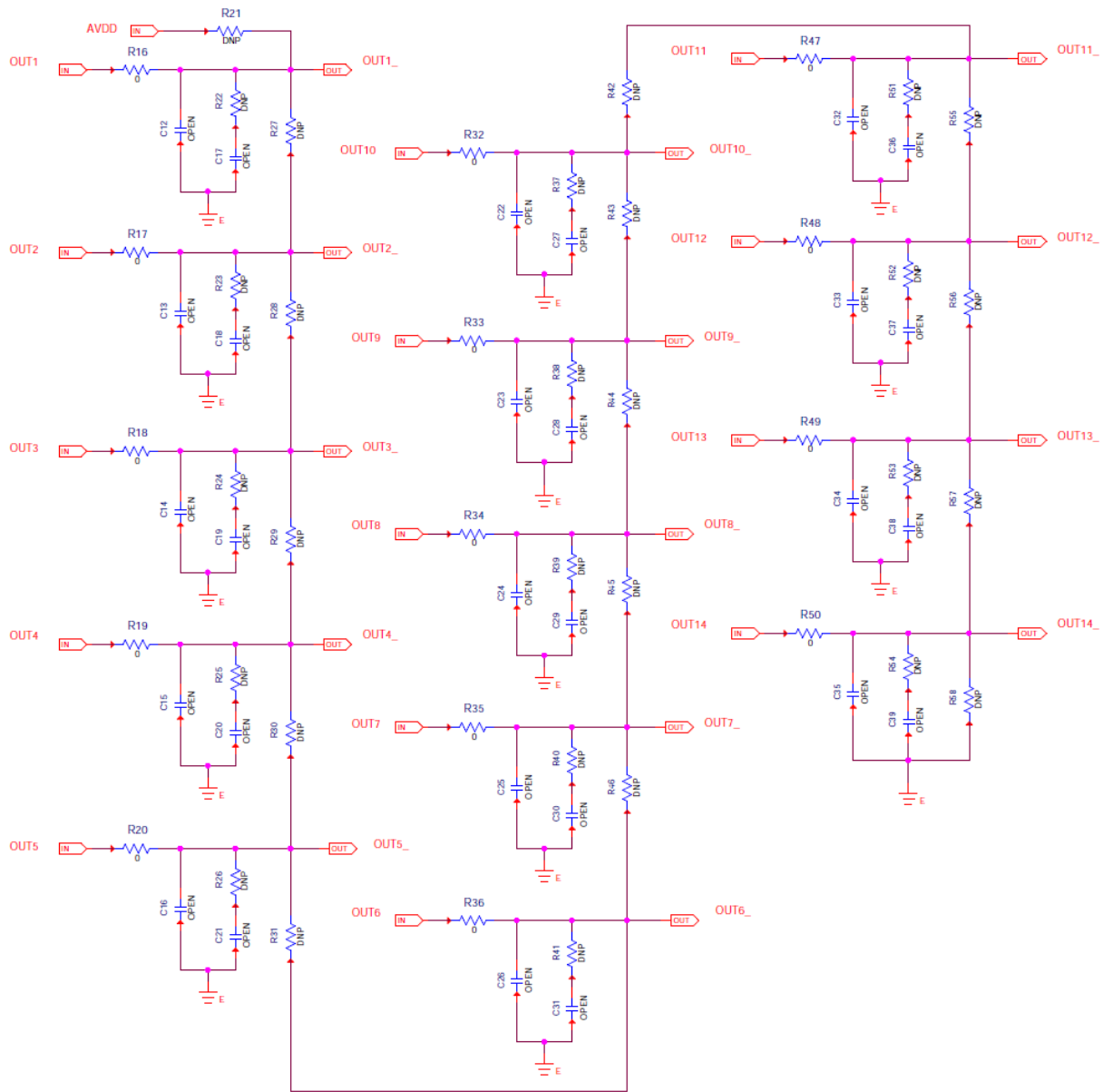
FIGURE 14. SCHEMATIC (Continued)
