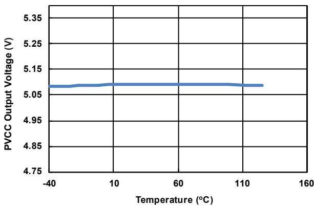
Figure 112. PVCC Output Voltage vs Temperature
