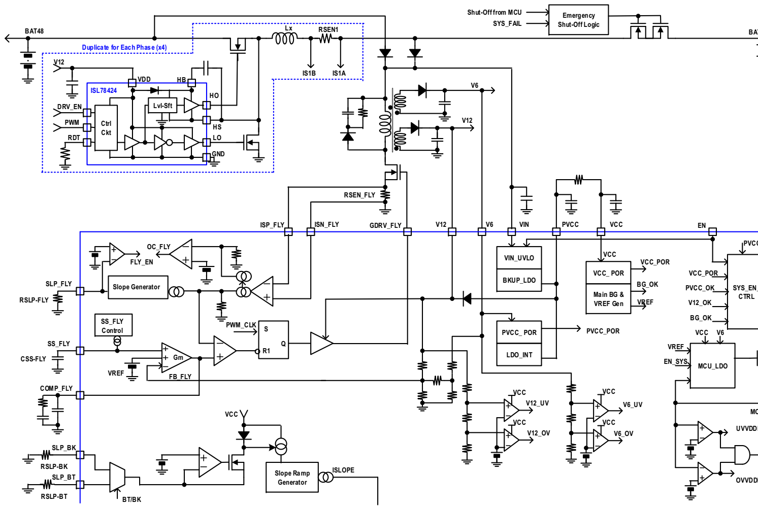
Figure 6. Block Diagram - Top
