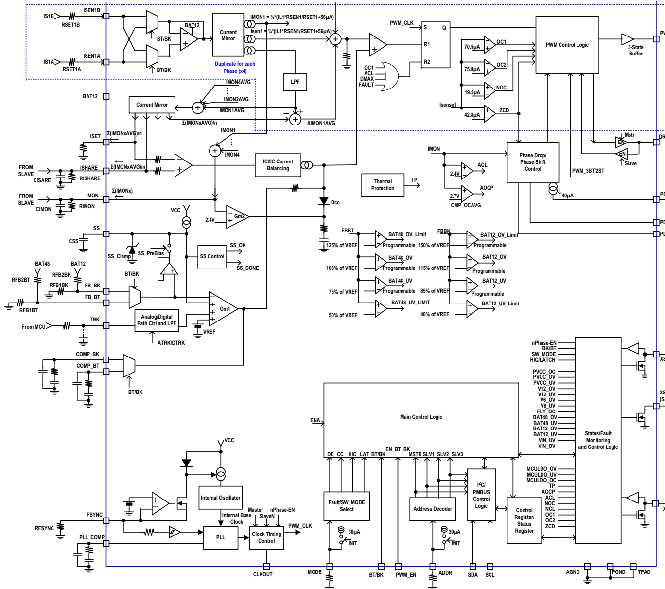
Figure 7. Block Diagram - Bottom
