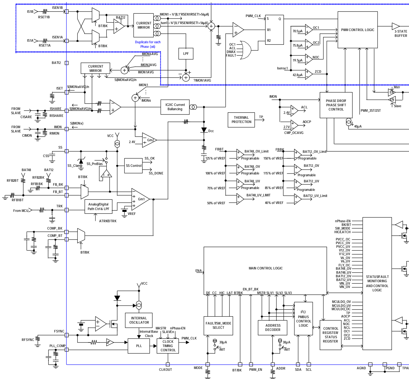
FIGURE 4. BLOCK DIAGRAM - BOTTOM
