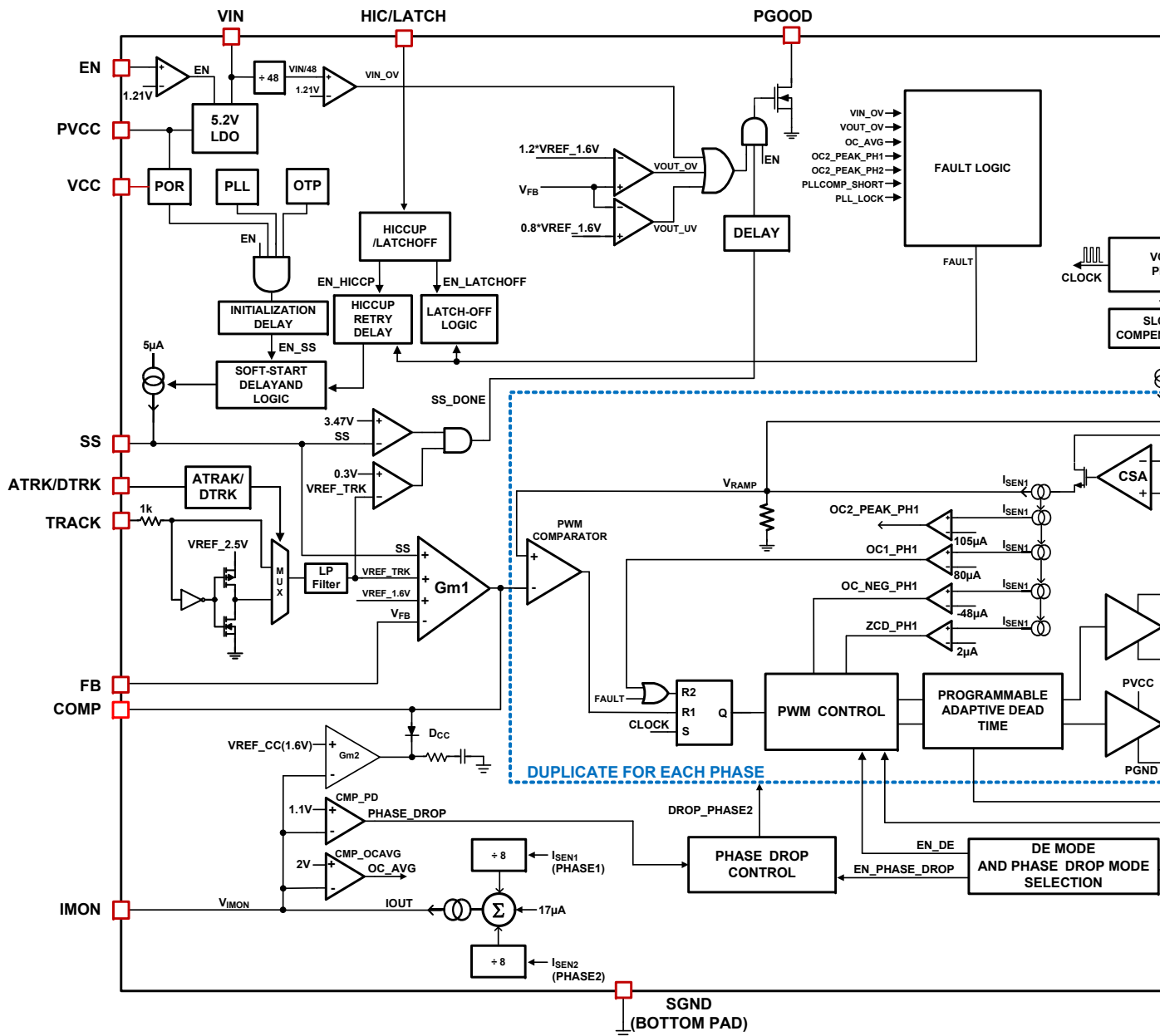
FIGURE 3. BLOCK DIAGRAM
