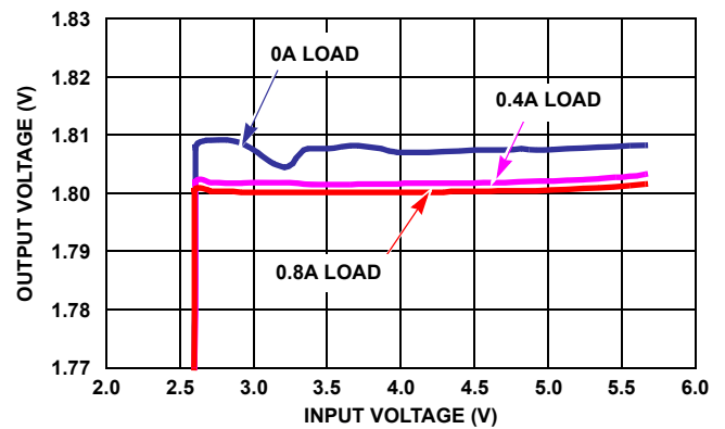
FIGURE 14. OUTPUT VOLTAGE REGULATION vs V_{IN} 1.8V_{OUT} PFM MODE
