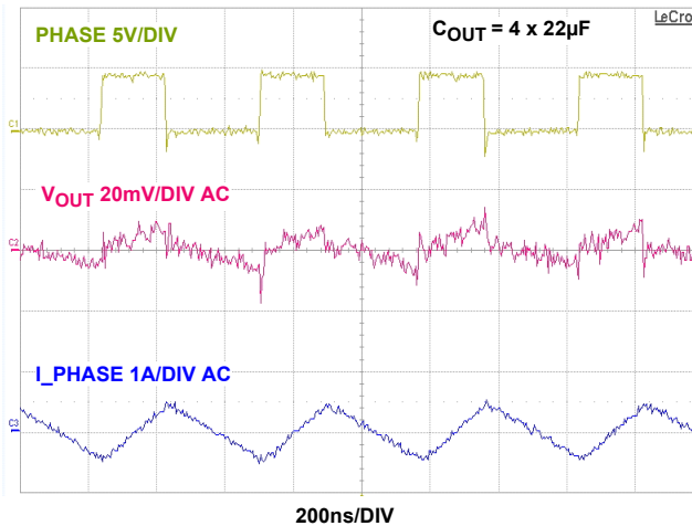
FIGURE 33. STEADY STATE AT 5A (SYNC = V_{DD} )
