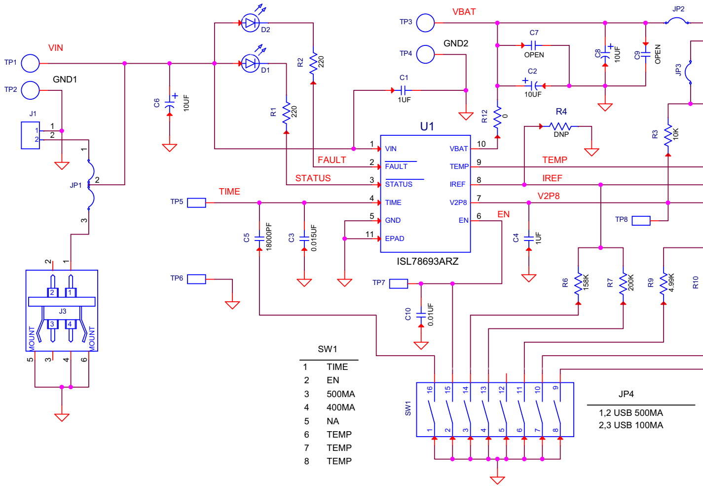
FIGURE 4. ISL78693EVAL1Z SCHEMATIC
