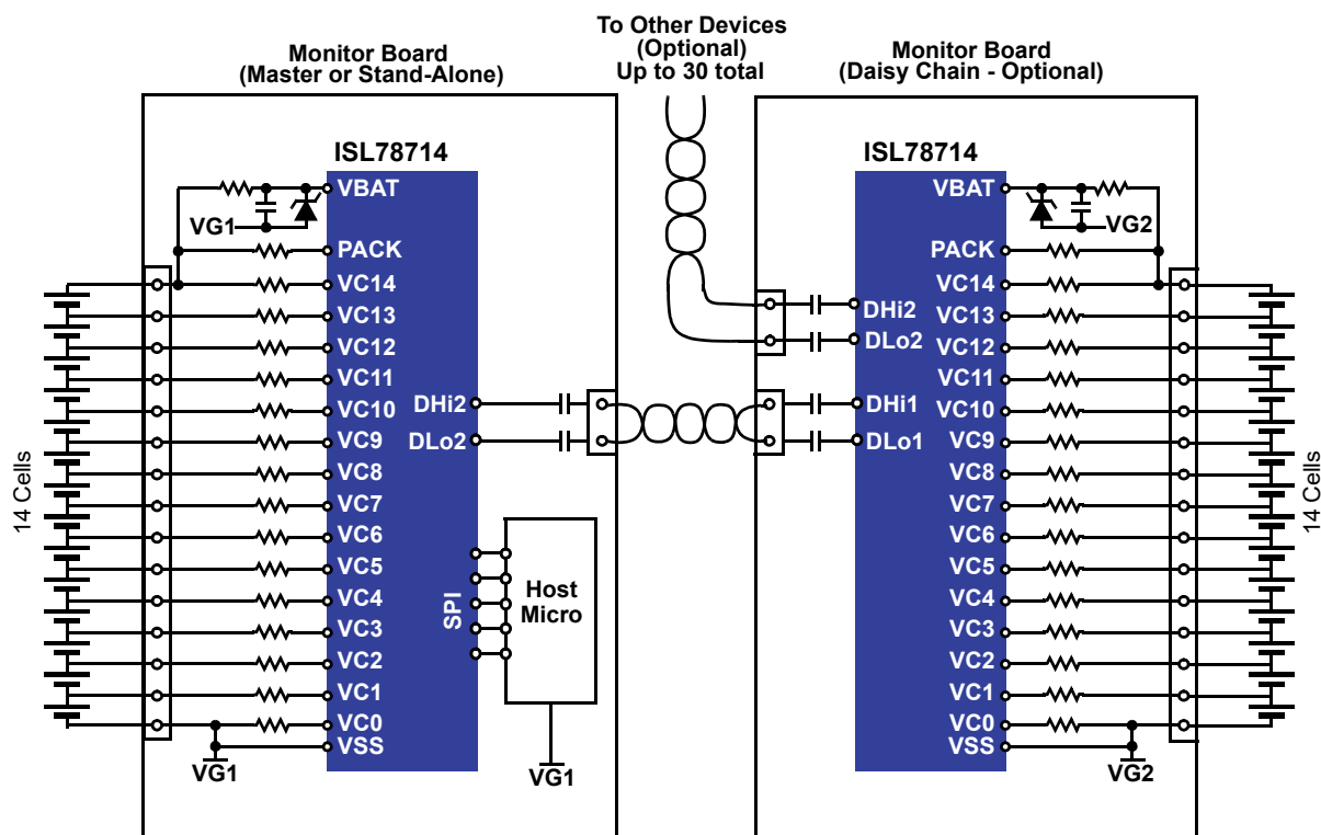
Figure 1. Typical Application
