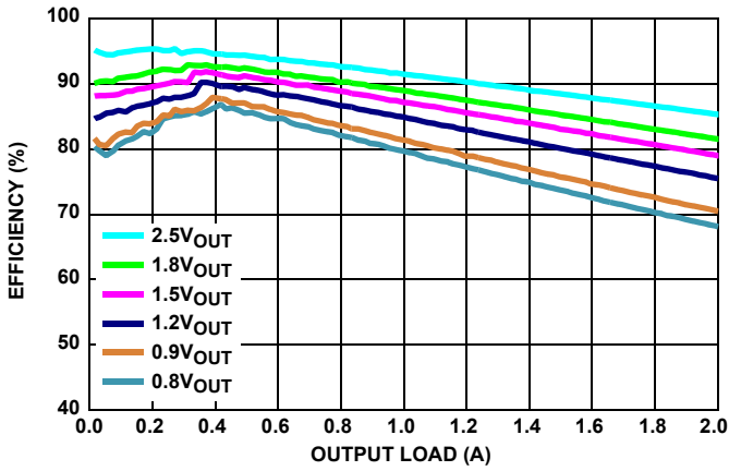
FIGURE 4. EFFICIENCY vs LOAD F_{SW} = 2MHz, V_{IN} = 3.3V, MODE = PFM, T_A = +25^\circ C
