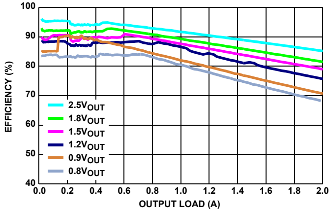
FIGURE 6. EFFICIENCY vs LOAD F_{SW} = 1MHz, V_{IN} = 3.3V, MODE = PFM, T_A = +25^\circ C
