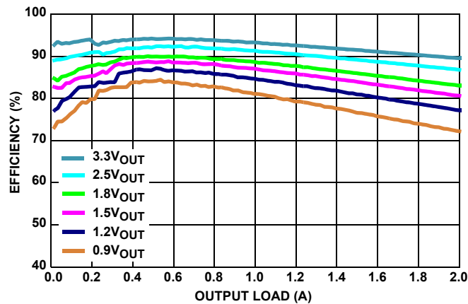
FIGURE 8. EFFICIENCY vs LOAD F_{SW} = 2MHz, V_{IN} = 5V, MODE = PFM, T_A = +25^\circ C
