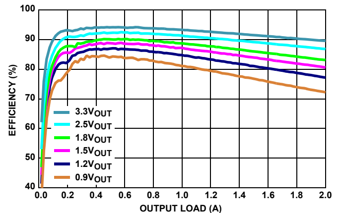
FIGURE 9. EFFICIENCY vs LOAD F_{SW} = 2MHz, V_{IN} = 5V, MODE = PWM, T_A = +25^\circ C
