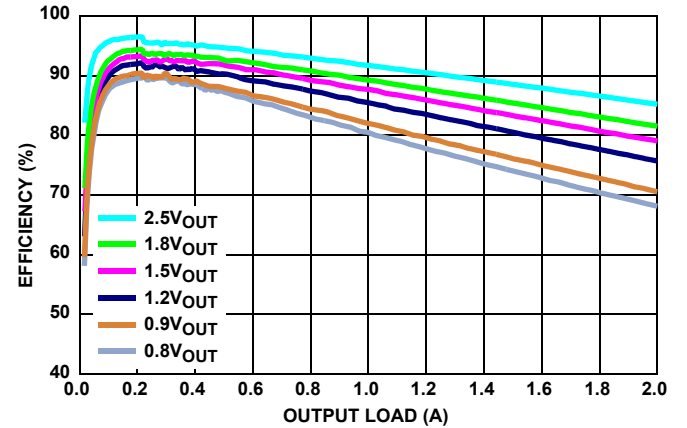
FIGURE 7. EFFICIENCY vs LOAD F_{SW} = 1MHz, V_{IN} = 3.3V, MODE = PWM, T_A = +25^\circ C
