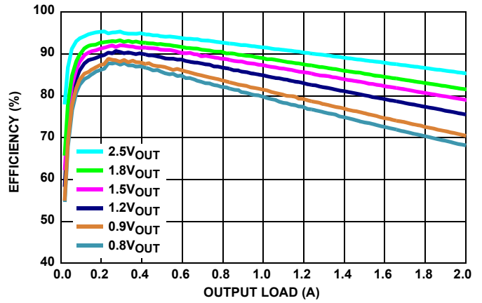
FIGURE 5. EFFICIENCY vs LOAD F_{SW} = 2MHz, V_{IN} = 3.3V, MODE = PWM, T_A = +25^\circ C
