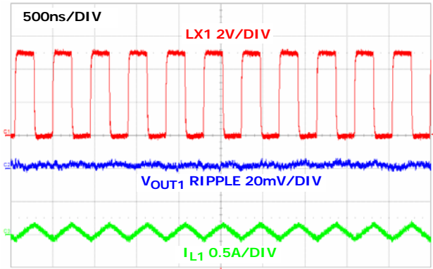
FIGURE 14. STEADY STATE OPERATION AT NO LOAD CHANNEL 1 (PWM)
