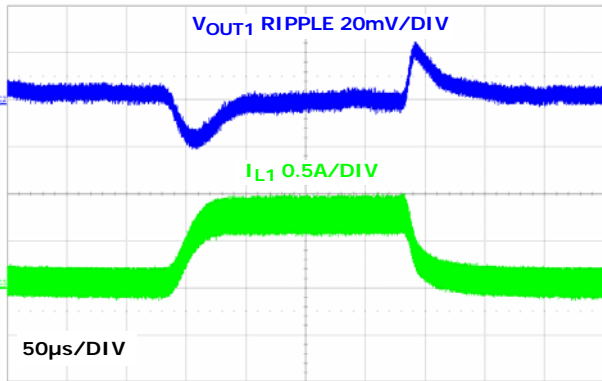
FIGURE 20. LOAD TRANSIENT CHANNEL 1 (PWM)
