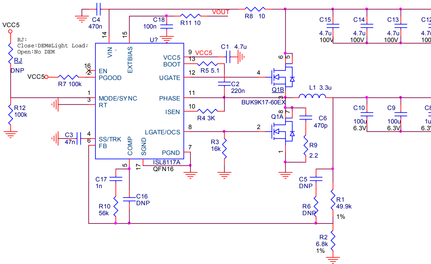
Figure 6. ISL8117ADEMO3Z Schematic
