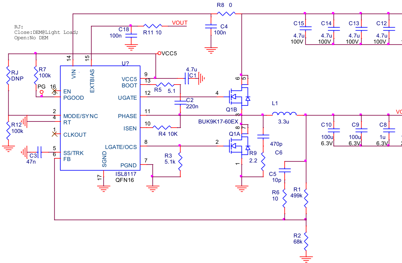
Figure 6. ISL8117DEMO4Z Schematic
