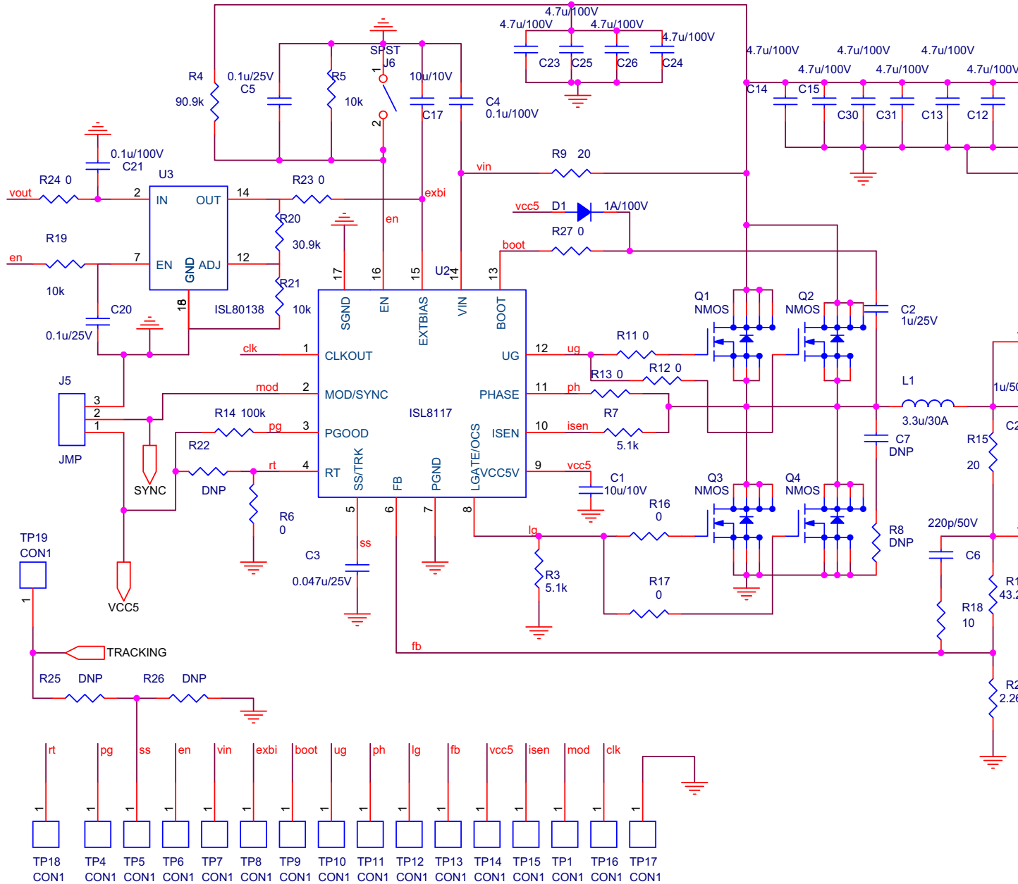
FIGURE 20. ISL8117EVAL2Z SCHEMATIC
