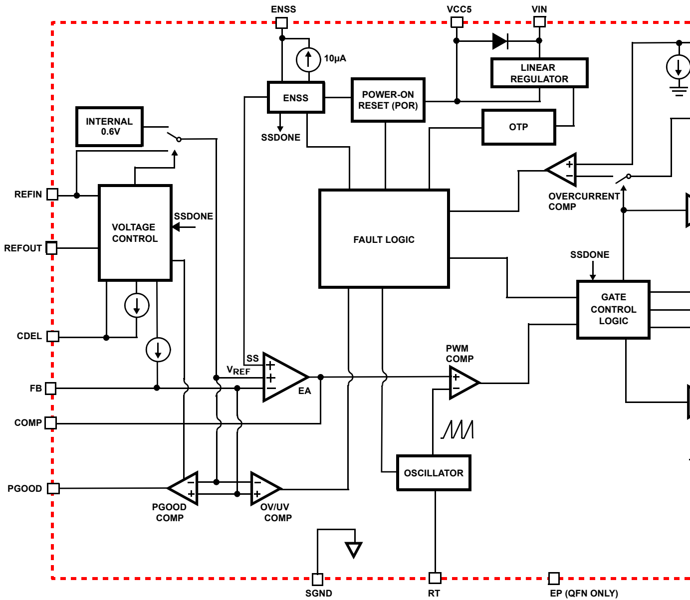
FIGURE 3. BLOCK DIAGRAM
