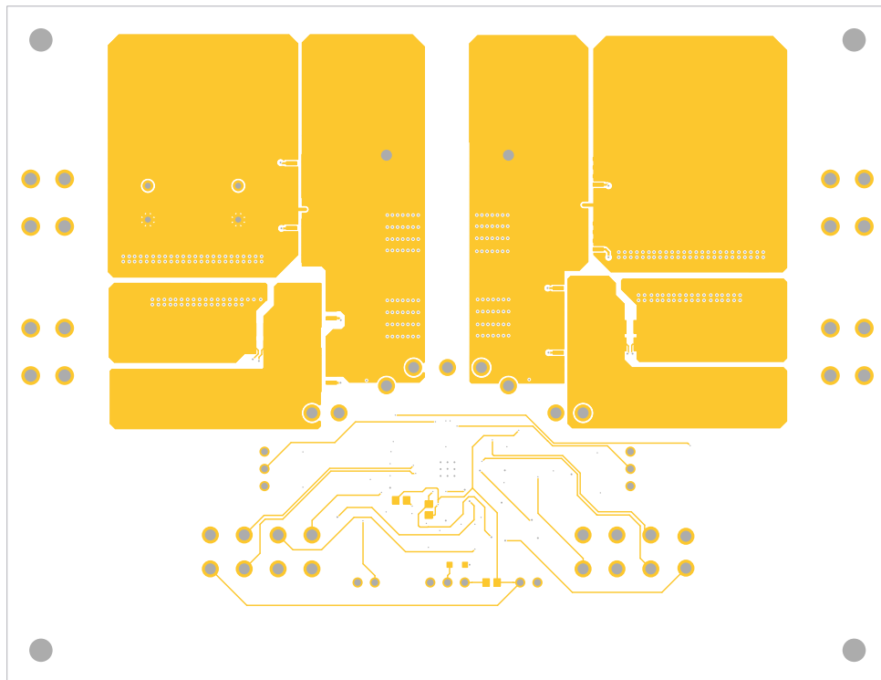
Figure 12. Bottom Layer
