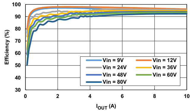
Figure 15. Efficiency, DEM
