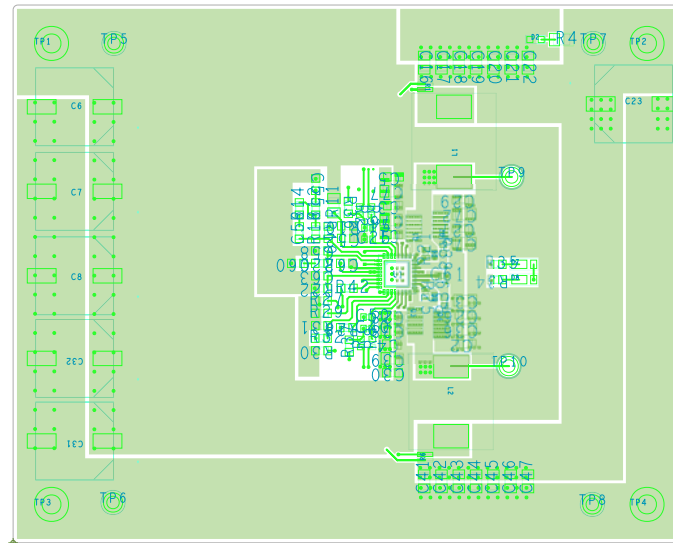
Figure 8. Top Layer
