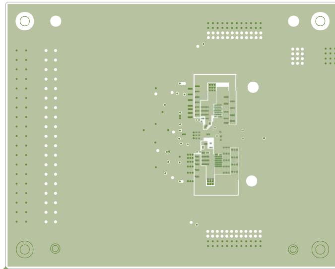
Figure 12. Fifth Layer
