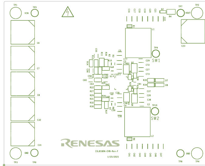
Figure 7. Silkscreen Top
