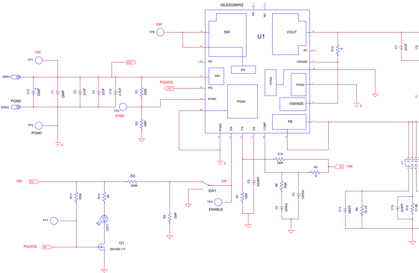
FIGURE 10. SCHEMATIC
