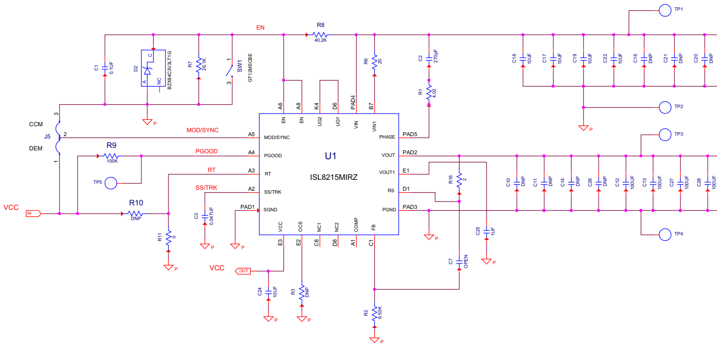
Figure 4. Schematic
