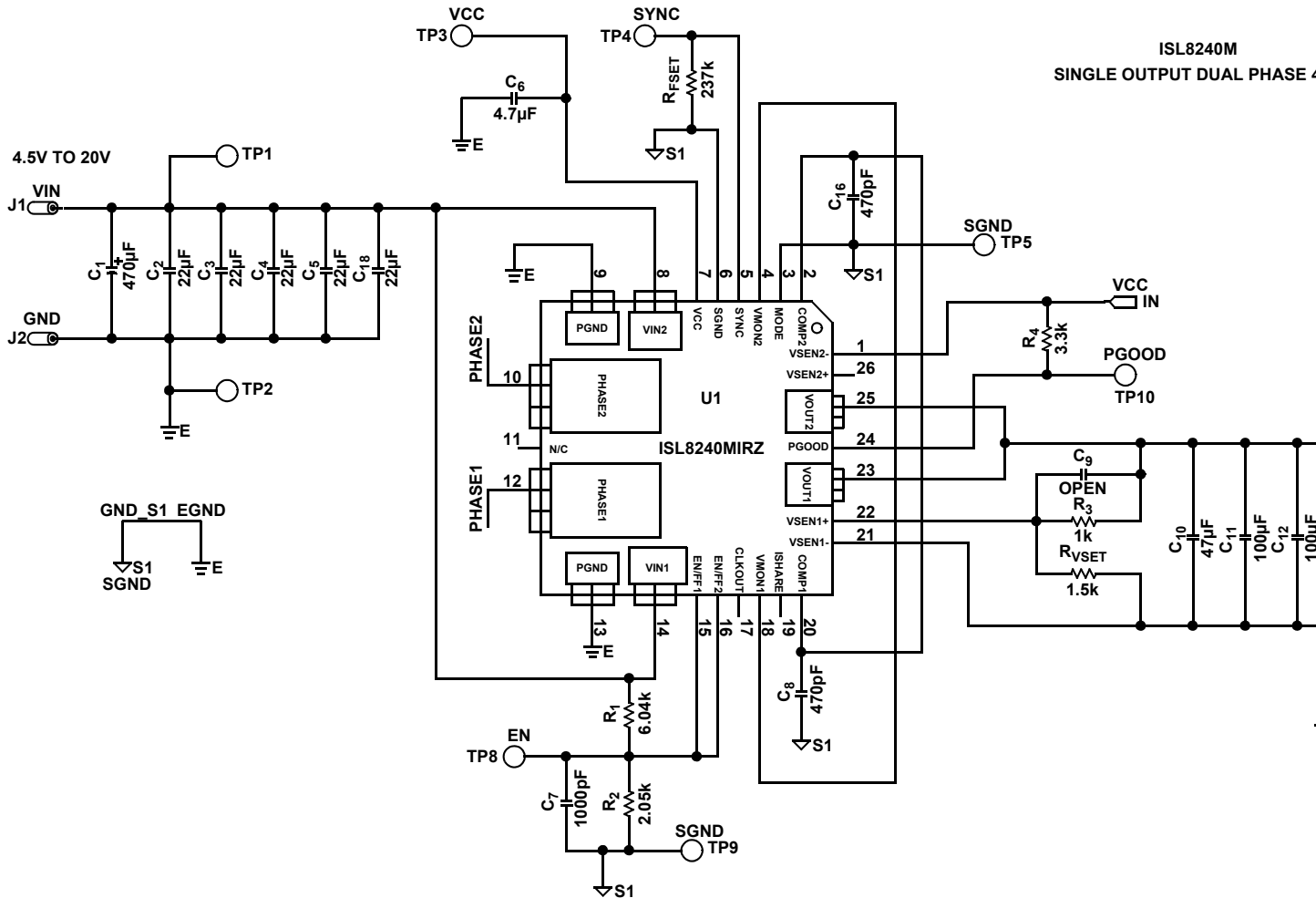
FIGURE 2. ISL8240MEVAL3Z BOARD SCHEMATIC
