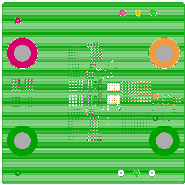
FIGURE 5. LAYER 2
