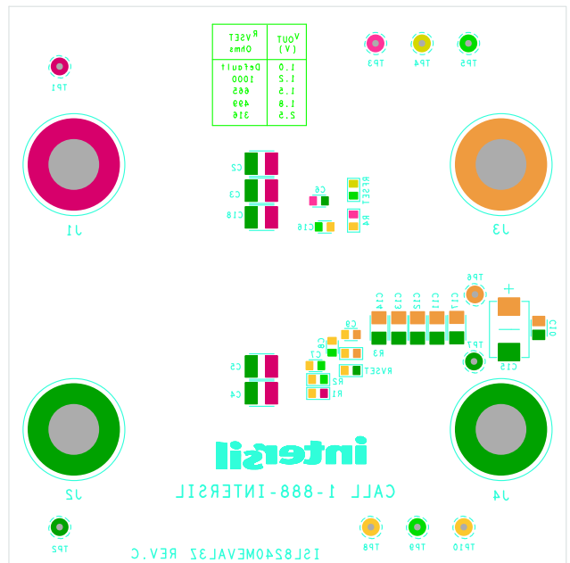
FIGURE 10. SILKSCREEN BOTTOM
