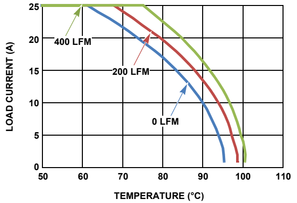
FIGURE 24. 12V_{\text{IN}} TO 3.3V_{\text{OUT}}
