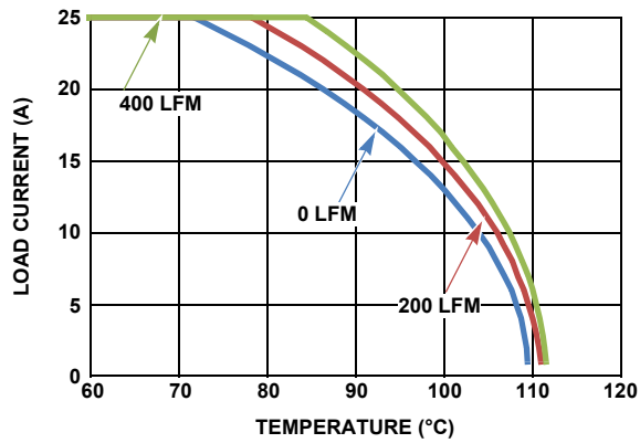
FIGURE 23. 5V_{\text{IN}} TO 3.3V_{\text{OUT}}
