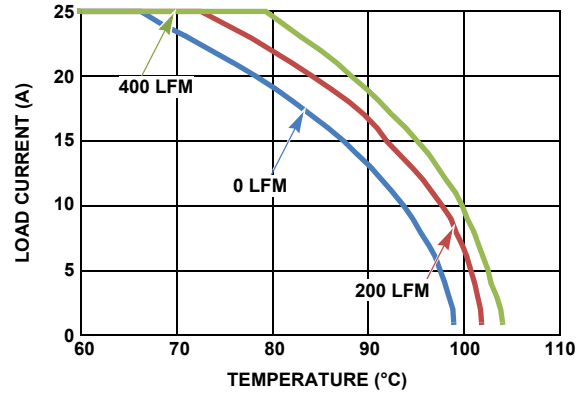
FIGURE 22. 12V_{\text{IN}} TO 2.5V_{\text{OUT}}
