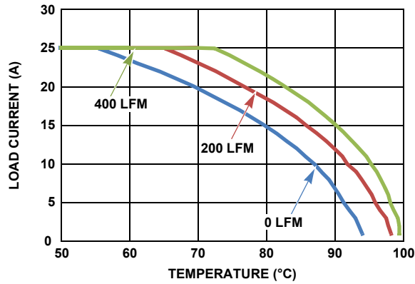
FIGURE 25. 12V_{\text{IN}} TO 5V_{\text{OUT}} , 727kHz
