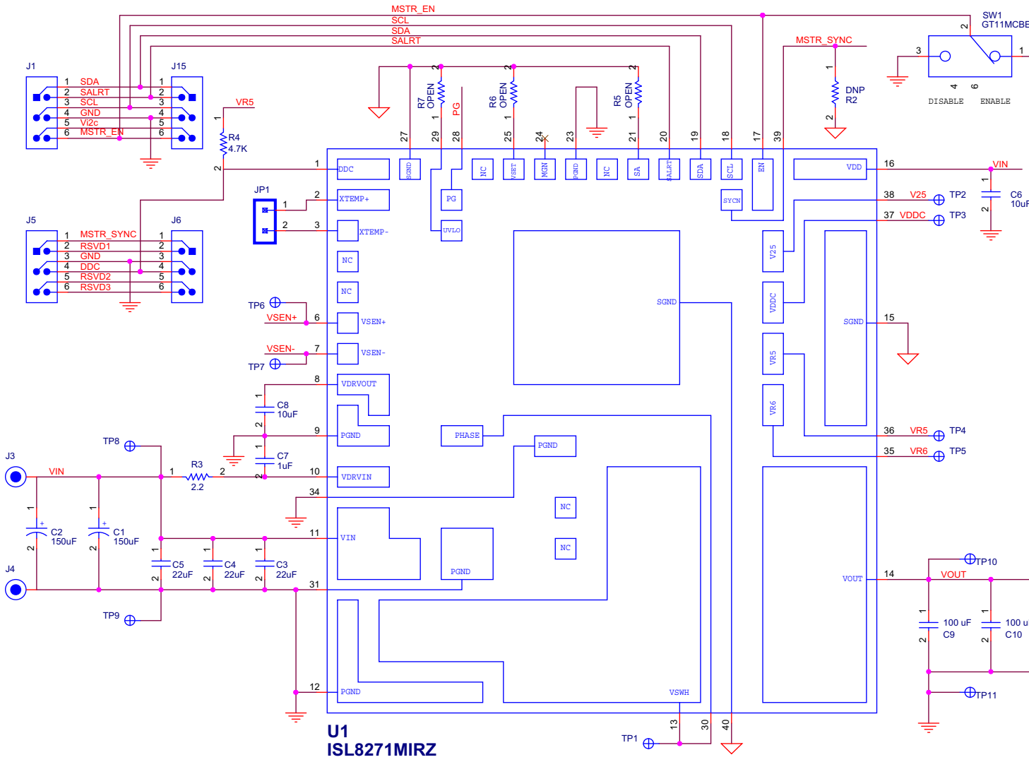
FIGURE 2. APPLICATION CIRCUIT
