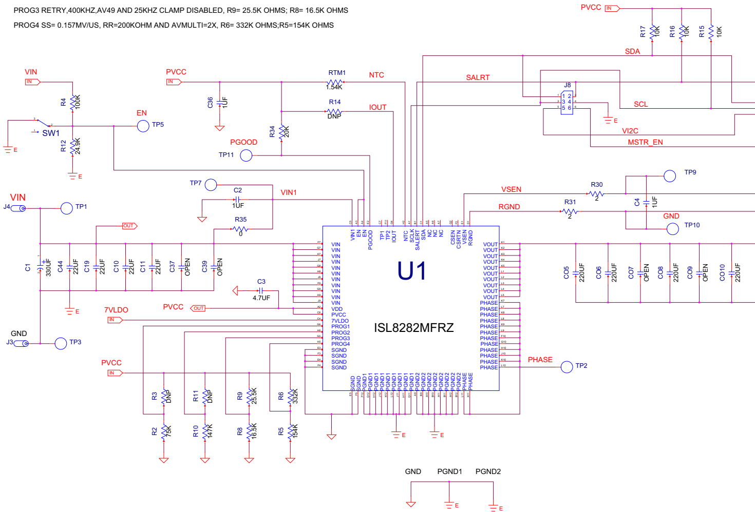
Figure 6. Schematic
