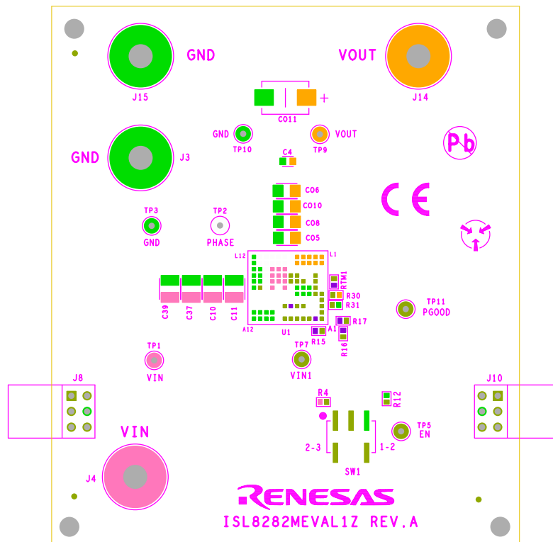
Figure 7. Silkscreen Top
