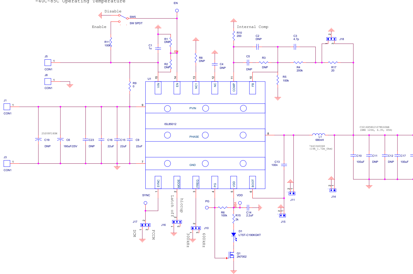
FIGURE 5. SCHEMATIC
