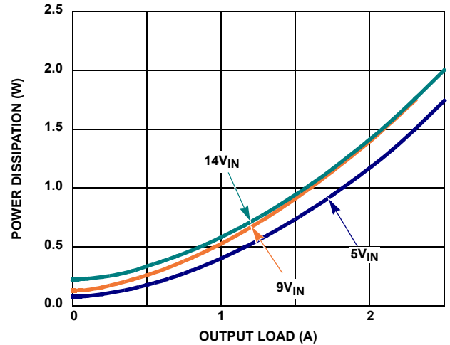
FIGURE 16. POWER DISSIPATION vs LOAD ( V_{OUT} = 2.5V , 500kHz)
