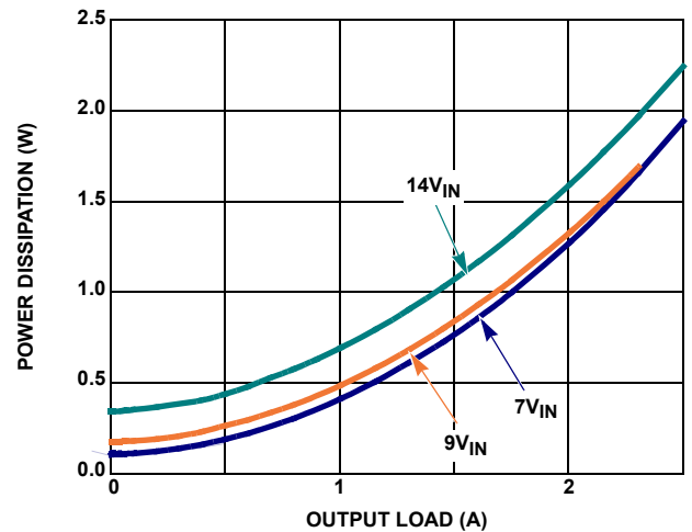
FIGURE 18. POWER DISSIPATION vs LOAD ( V_{OUT} = 5V , 500kHz)
