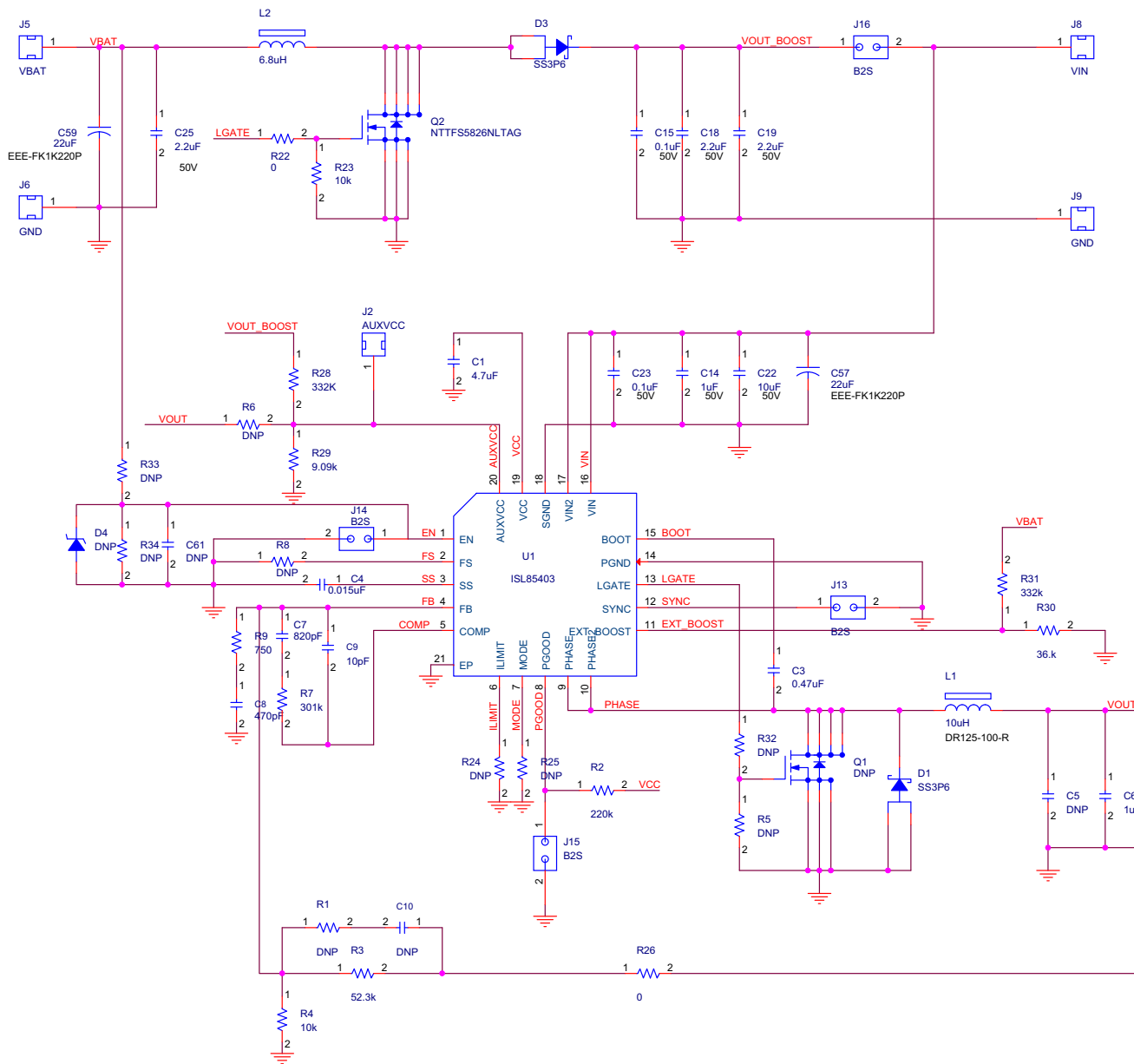
FIGURE 5. ISL85403EVAL1Z SCHEMATIC
