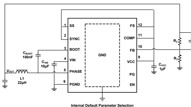
Figure 1. Typical Application
