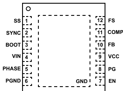
12 Ld 4x3 DFN Top View
