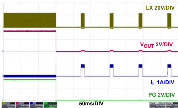
FIGURE 29. OVERCURRENT PROTECTION HICCU, PWM
