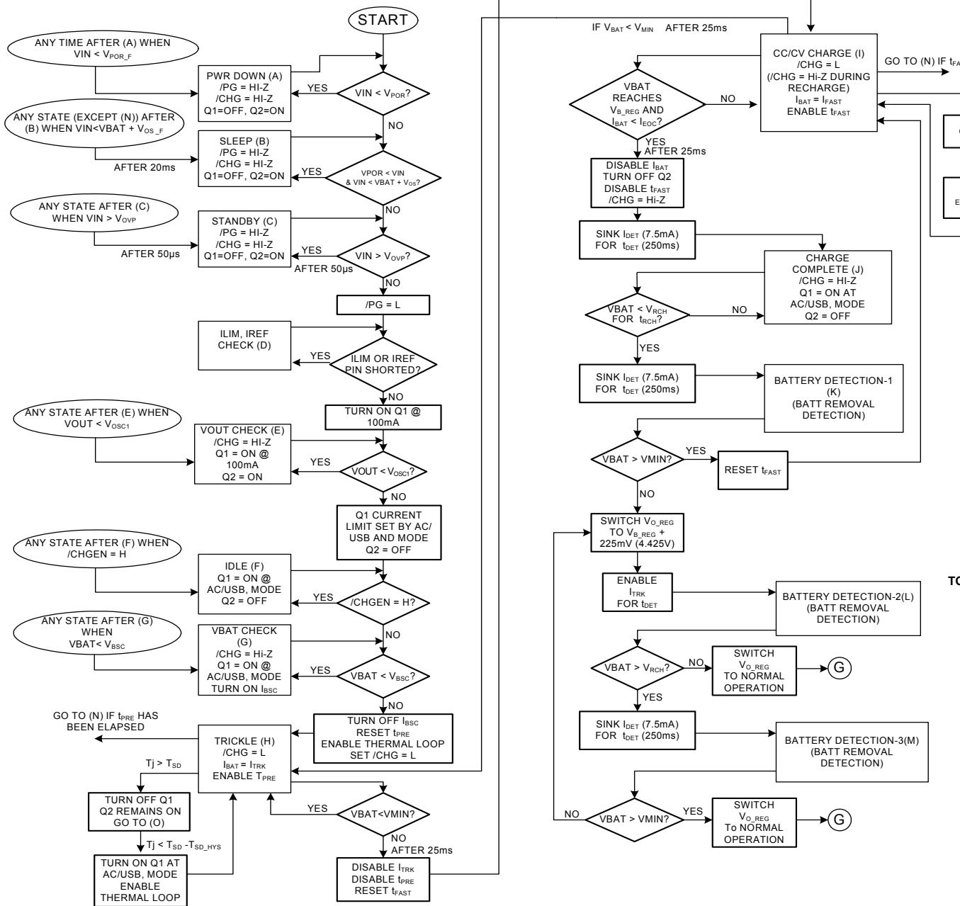
FIGURE 32. STATE DIAGRAM (CONT = L)
