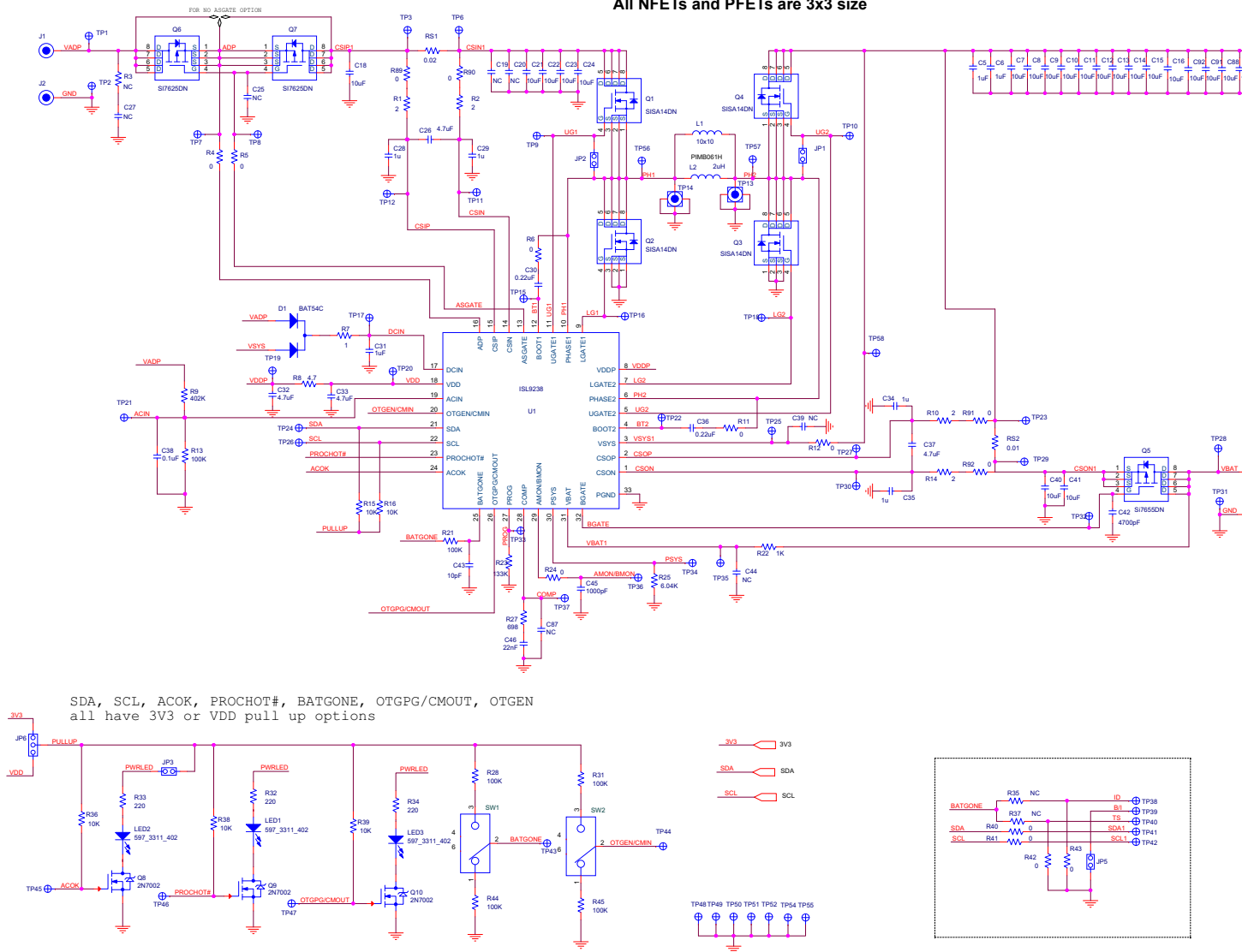
FIGURE 6. ISL9238EVAL1Z BOARD SCHEMATIC
