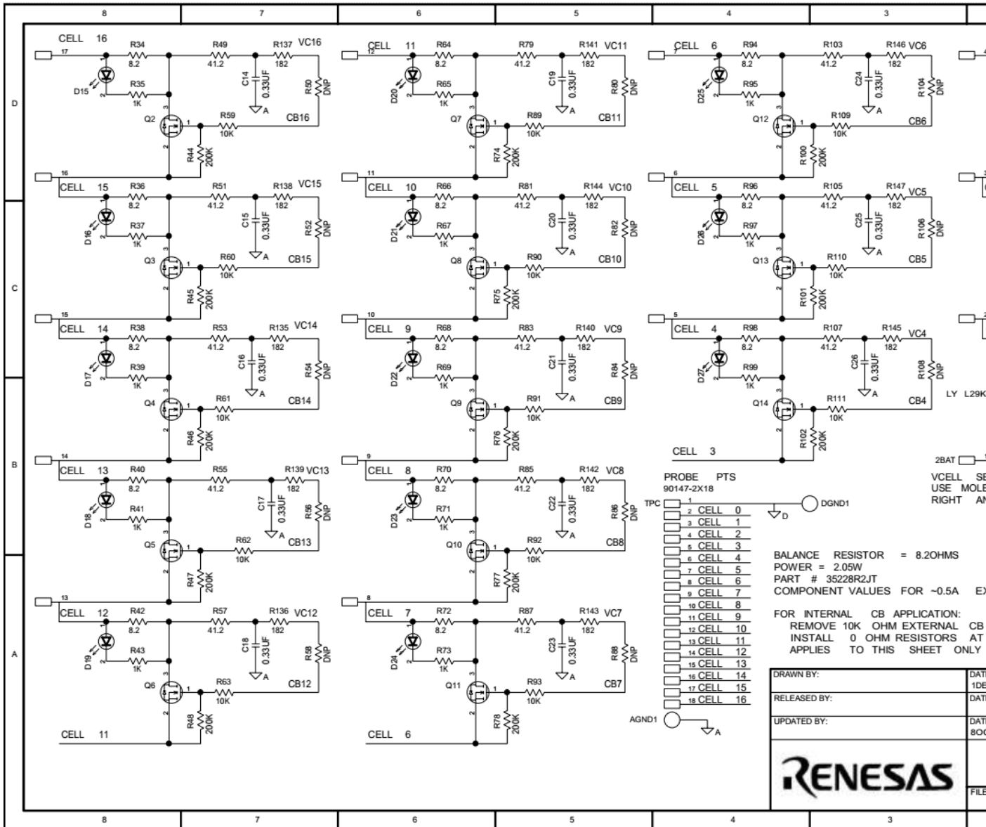
Figure 71. Eval Board Schematic Sheet 2
