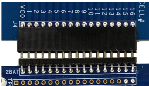
Figure 9. Cell Connection
