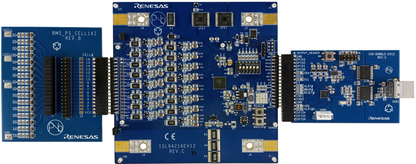
Figure 8. BMS Assembly
