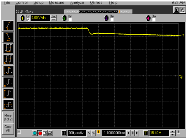
FIGURE 10. VLNB TRANSITIONS FROM 18.3V TO 13.3V
