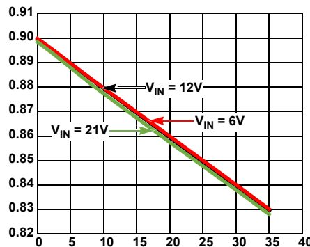
Figure 2. V_{GT}/VR B Load Line = 2mΩ
