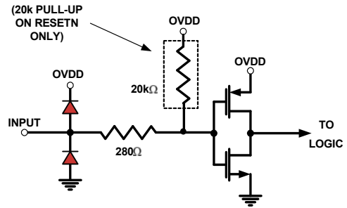
FIGURE 51. DIGITAL INPUTS
