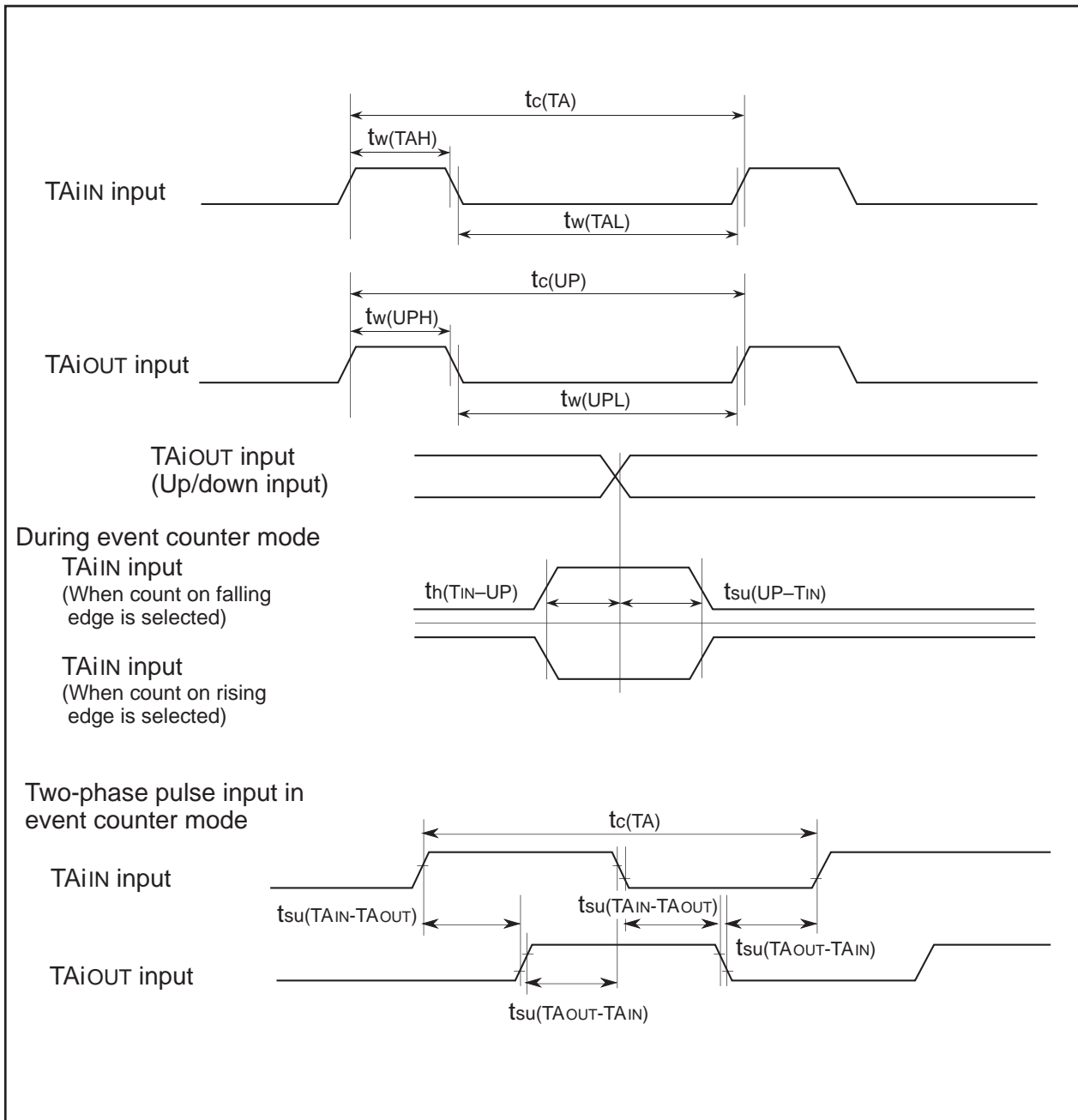
Figure 1.19.1. Timing Diagram (1)
